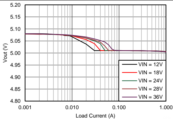
Figure 61. Output Voltage Regulation
