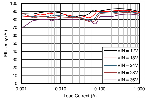
Figure 60. Efficiency
